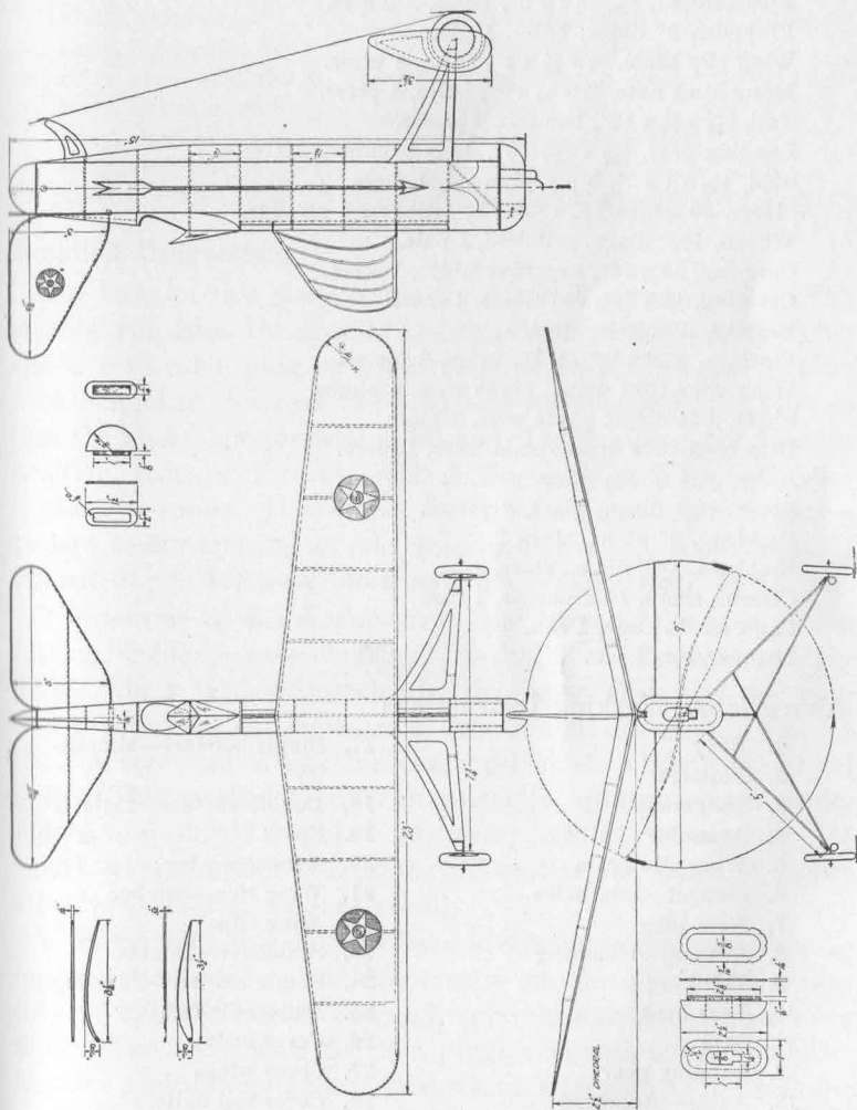
Fig. 85—3-Plan Drawing—Sky Pursuit
